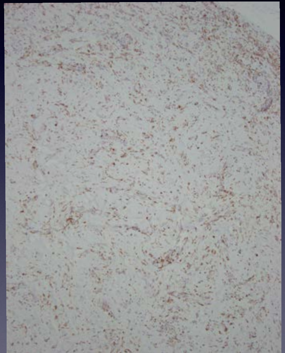
CD68
